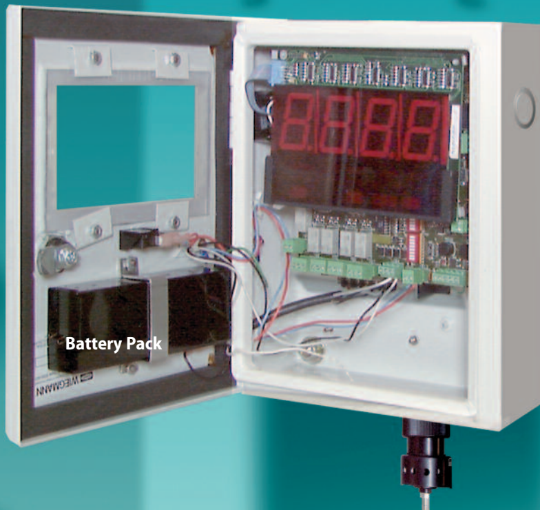
Bottom-Mount Sensor
